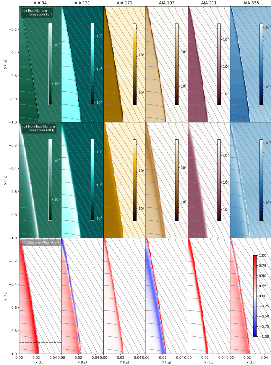
Figure 6. Synthetic SDO/AIA images for Case A2 applying conduction flux-limitation. The panels are defined as same as in Figure 5.
