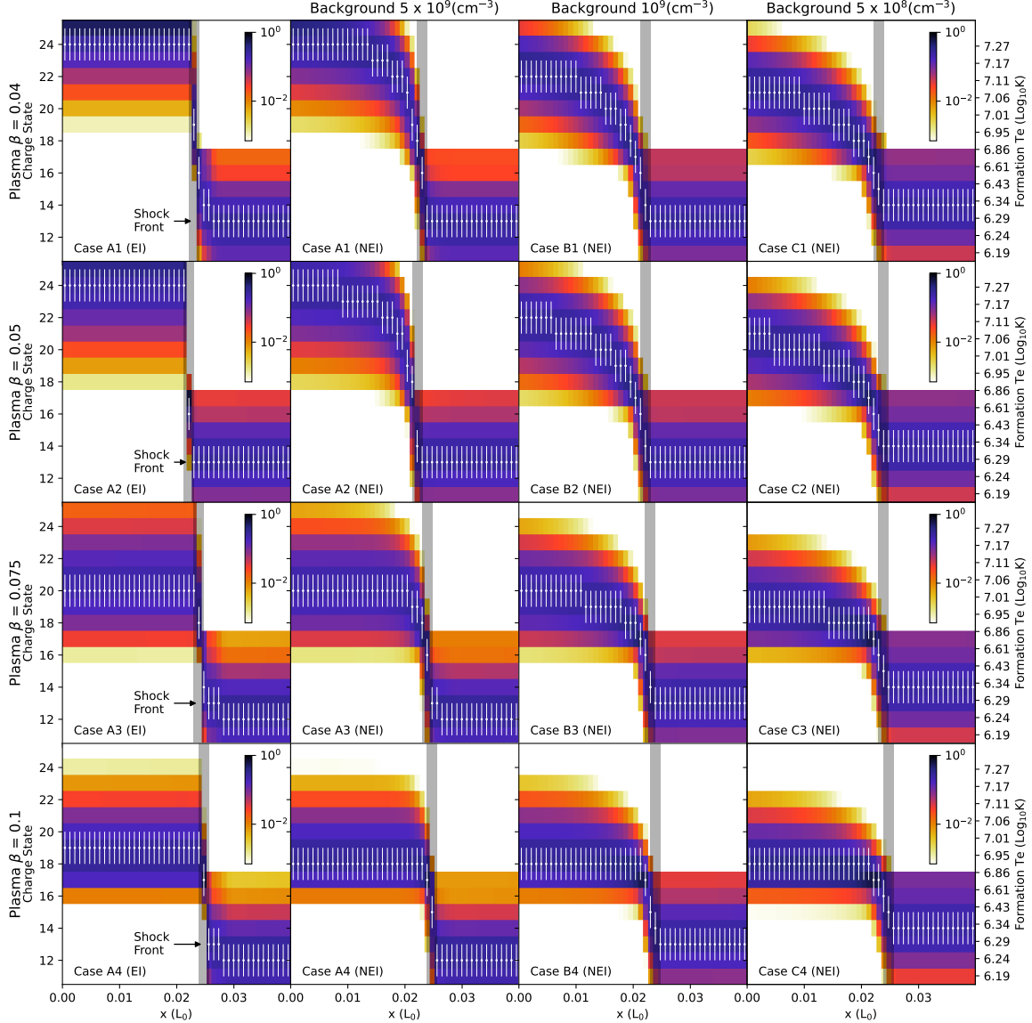
Figure 3. Fe ion fractions along the sampling line ( y=-0.9L_0 , as same as in Figure 1(a)) in different cases. The left panel shows the equilibrium ionization results of Case A series, and the right three panels are for NEI situations with different background coronal density 5 \times 10^9 , 10^9 , and 5 \times 10^8 \text{cm}^{-3} , respectively. From top to bottom, each row is for the different plasma \beta , 0.04, 0.05, 0.075, and 0.1, which are relative to the post-shocked plasma temperatures around 18 MK, 16 MK, 10 MK, and 8 MK. The white vertical bars indicate the most dominant top three ions along the sampling line at each position. The right axis labels the corresponding formation temperature of each ion assuming ionization equilibrium.
