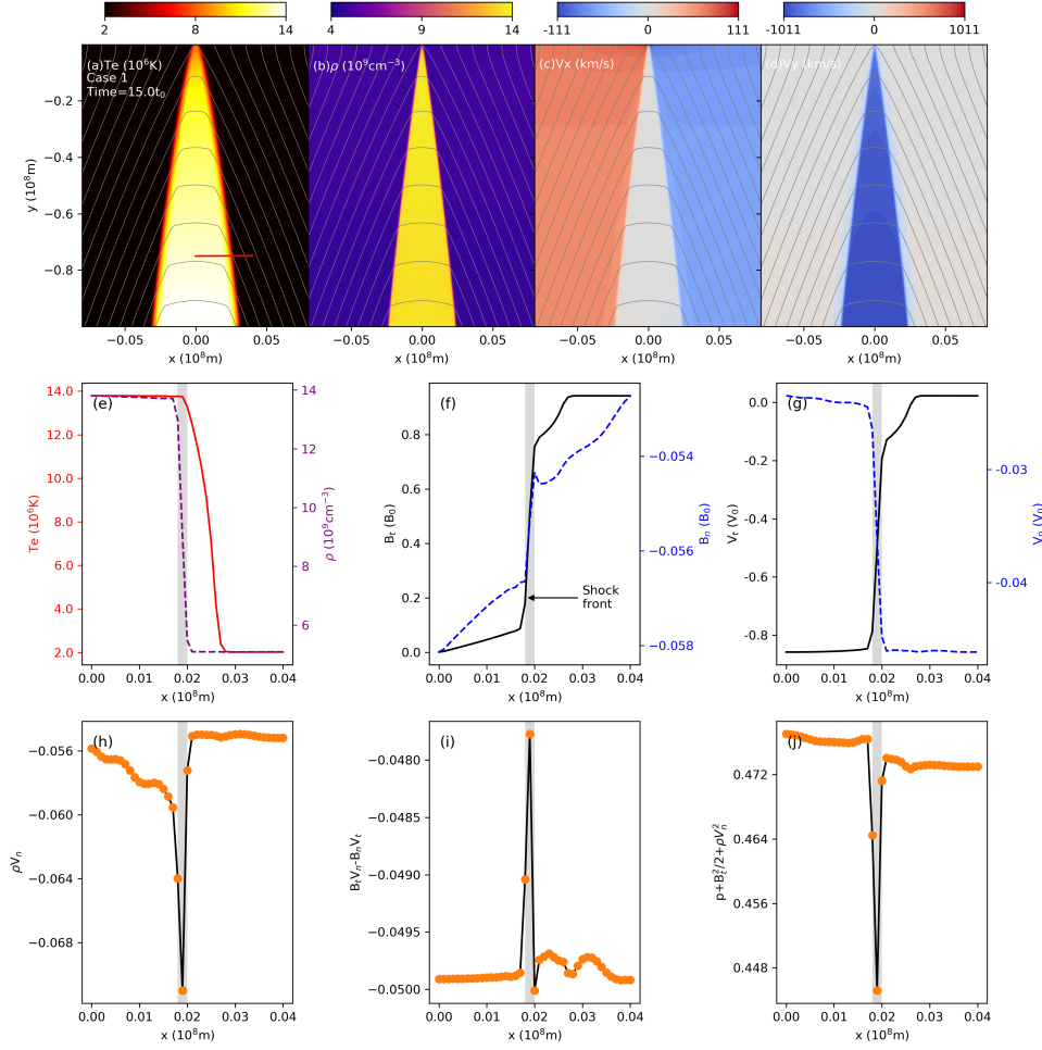
Figure 16. The slow-mode shocks in a Petschek-type reconnection simulation with the classical Spitzer thermal conduction coefficients. (a-d) The temperature, density, plasma velocity around the reconnection X-point, and a pair of slow-mode shocks. The solid gray contours are for magnetic field lines. (e-g) Primary variables distribution crossing the shock front along the red sampling line shown in the panel (a). The vertical gray shadows indicate the position of the shock front. Here B_t (and V_t ) is the transverse component of magnetic field (and velocity), and B_n (and V_n ) is the normal component to the shock front, respectively. (h-j) Non-dimensional mass flux, magnetic flux, and energy flux distribution that continues crossing the slow mode shocks.
