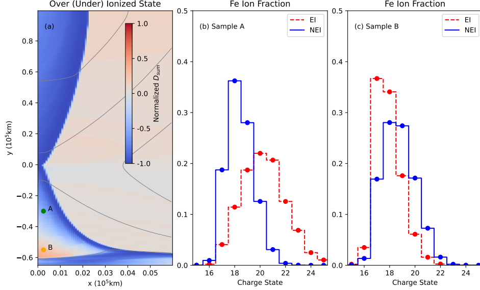
Figure 10. Under-ionized and over-ionized ionization states in downwards outflow regions. Panel (a) shows the normalized total difference ( D_{sum} ) between NEI fraction and EI assumption; (b) and (c) are Fe ion populations at two chosen sampling points indicated by green and orange cycles in panel (a), respectively.
