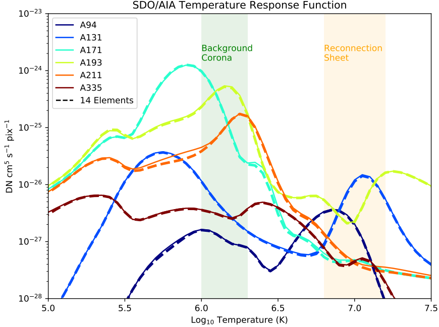
Figure 17. Temperature response function for six SDO/AIA channels. The solid lines are calculated from the Chianti database (Dere et al. 2019) assuming ionization equilibrium and the coronal abundance (Feldman 1992). The dotted lines counts the most abundant 14 elements (H, He, C, N, O, Ne, Mg, Al, Si, S, Ar, Ca, Fe, and Ni) calculated in this work. The green and orange shaded regions indicate the temperature ranges of the background corona and reconnection current sheets, respectively.
