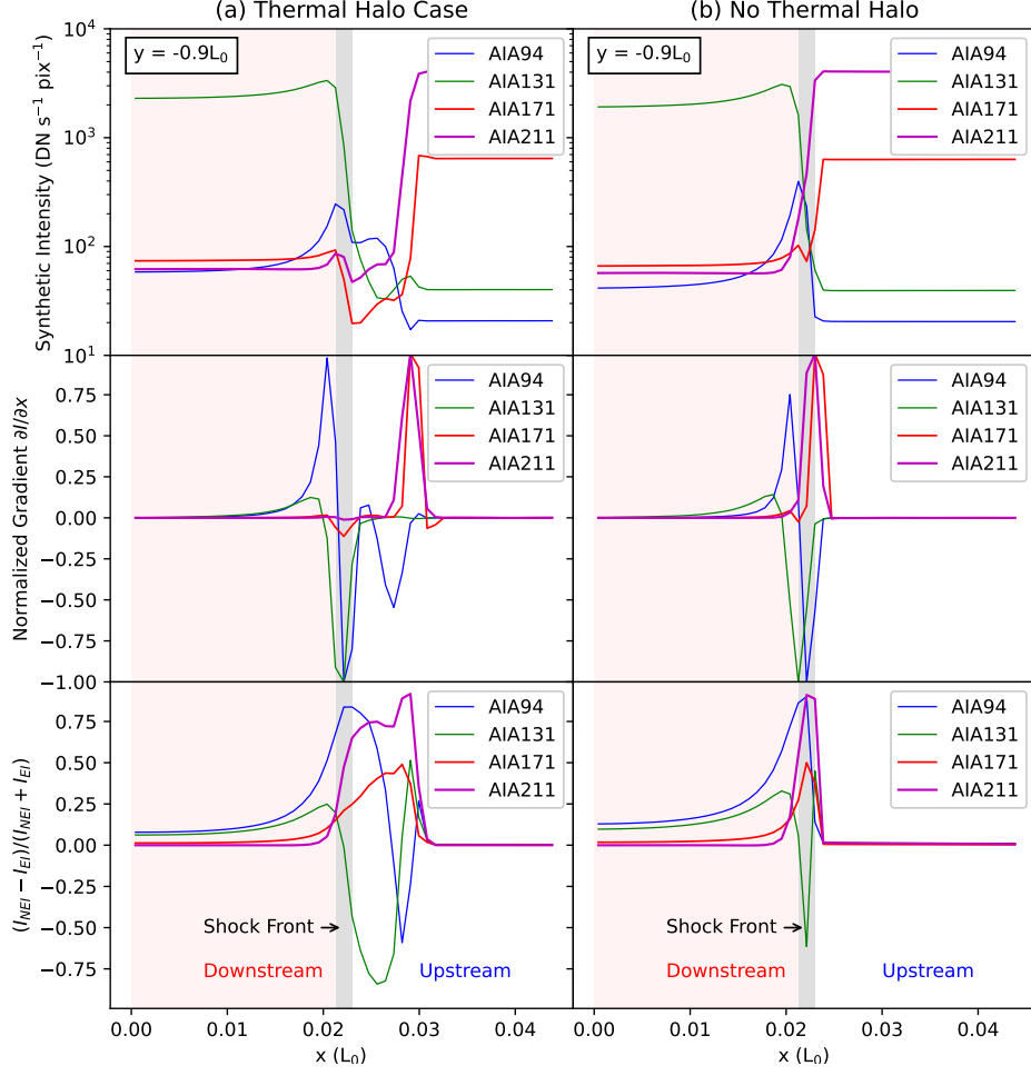
Figure 7. Synthetic SDO/AIA intensity in NEI around the shock front along the horizontal sampling line at y = -0.9L_0 as shown by dashed line in Figures 5 and 6. The left panels (a) are for Case A2* with the thermal halo, and the right panels (b) are for Case A2 without the thermal halo, respectively. The top rows are emission intensity ( I ), the middle rows are normalized intensity gradient in x - direction \partial I/\partial x , and the third row are predicted intensity difference between NEI and EI results, (I_{nei} - I_{ei})/(I_{nei} + I_{ei}) .
