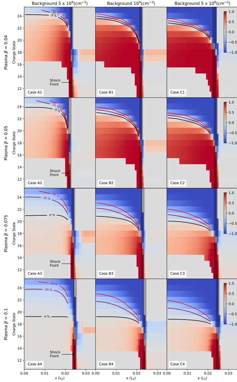
Figure 4. The relative difference of Fe ion population between NEI and equilibrium ionization, defined by f_{diff} = (f_{nei} - f_{ei}) / (f_{nei} + f_{ei}) . The colored solid lines marked the position with f_{diff}=0 , -25\% , and -50\% .
