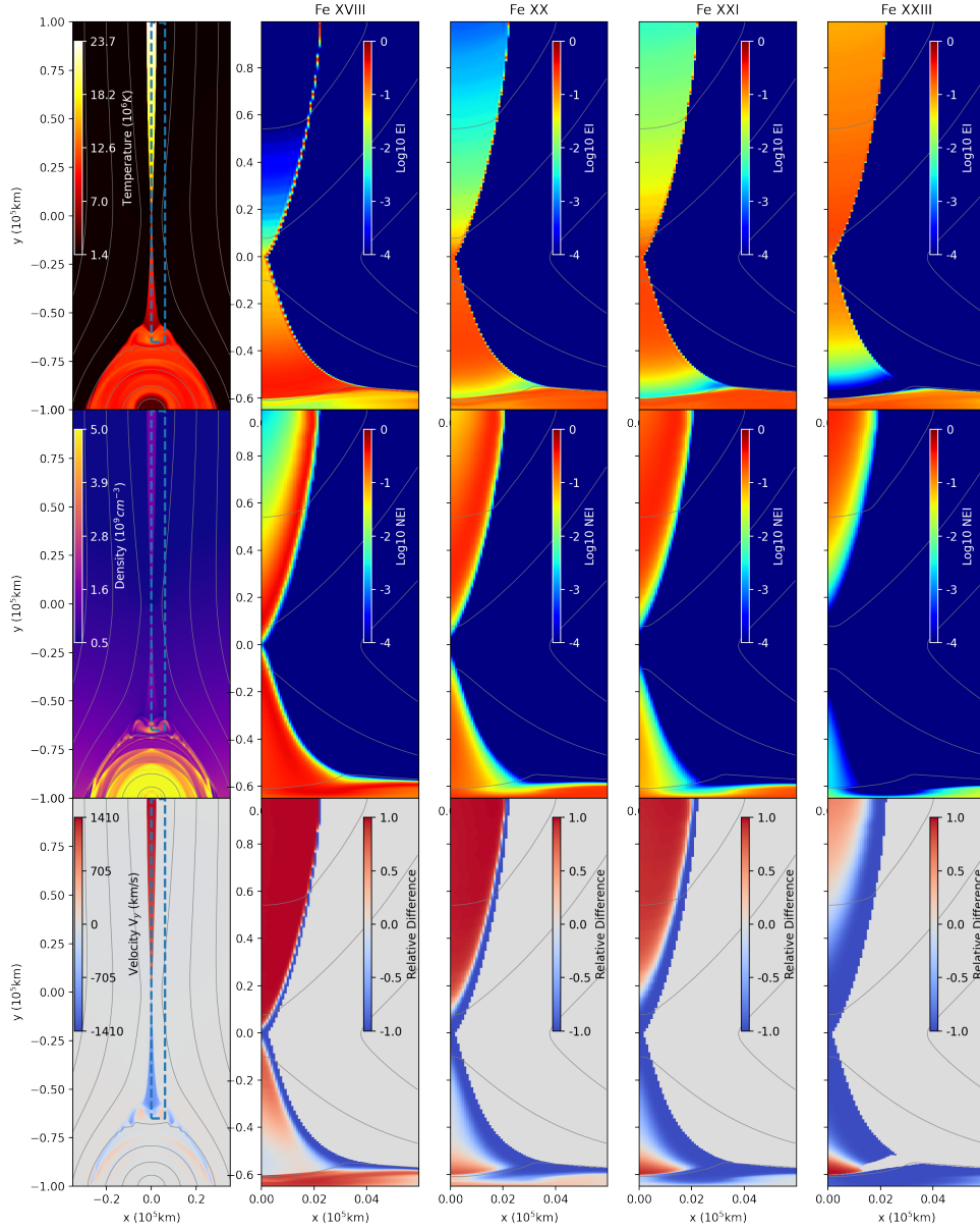
Figure 9. Ionization distribution with the line-tied boundary condition in Case D. The left panel shows the distributions of temperature, density, and velocity component V_y at the time t = 16t_0 . The right panels are ion fraction of Fe XVIII, Fe XX, Fe XXI, and Fe XXIII in the local region shown by the blue box on the left panels. The top row is ion fractions in the equilibrium ionization ( f_{ei} ), the second row is for NEI ( f_{nei} ), and the third row shows relative differences between NEI and EI defined by (f_{nei} - f_{ei})/(f_{nei} + f_{ei}) .
