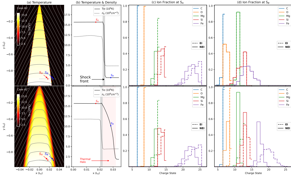
Figure 1. Temperature and density distribution across the Petschek-type shocks in Case A2 and A2*. Here, Case A2 employed the conductive flux-limitation and Case A2* is for the classical Spritzer conduction simulation. Two sampling points ( S_A , S_B ) have been chosen along the dotted horizontal sampling line at y = -0.9L_0 . Here, the non-dimensional characteristic length L_0 = 1.5 \times 10^8 m. Panels (b) are temperature and density profiles along the sampling line shown in (a). The gray and red shaded regions indicate the shock front and thermal halo regions, respectively. Panels (c-d) show ion fractions of C, O, Mg, Si, and Fe at S_A and S_B . The solid lines show the NEI results, and the dashed lines are for equilibrium ionization. The charge state in the horizontal axis is in spectroscopic notation in which Fe XII means Fe ^{11+} .
