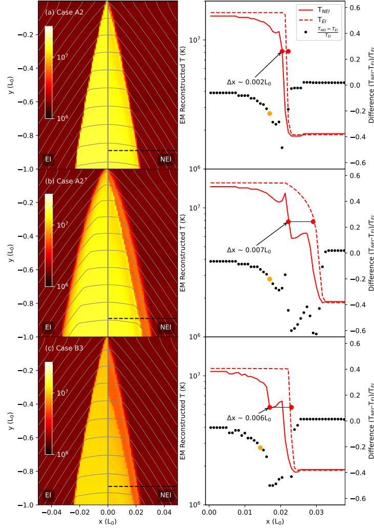
Figure 8. Emission measure reconstructed temperature distribution using the synthetic SDO/AIA intensity for Case A2, A2*, and B3. In each temperature map, the left region ( x ranges from -0.05 to 0 ) shows the MHD modeled temperature (or temperature in EI), and the right part ( x ranges from 0 to 0.05 ) is for the reconstructed temperature. The right panels are temperature distribution, and the relative difference between NEI and EI results along the horizontal sampling line at y = -0.9L_0 (dashed black lines on the left panels). The two red dots mark the location of the half-maximum temperature, and \Delta x indicates the distance between the above two red cycles in x -direction. The orange dot indicates the position with \sim 20\% difference along the dotted lines.
