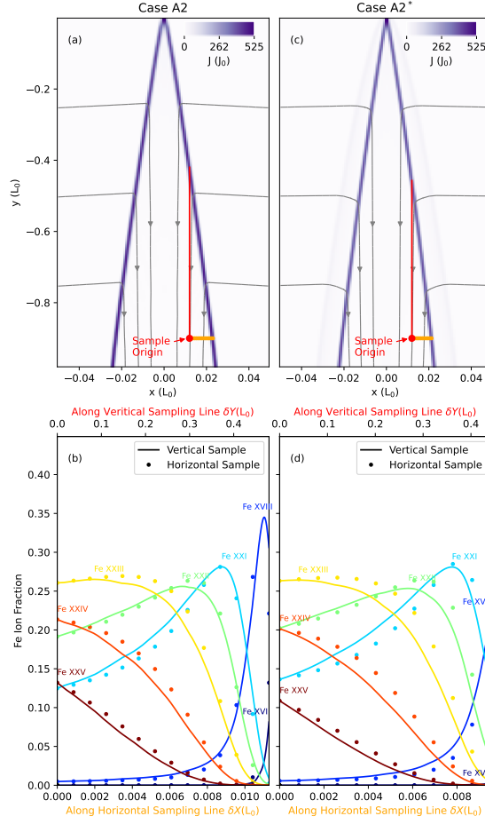
Figure 2. Iron ion fraction distribution across Petschek-type shocks in Case A2 and A2*. In the top panels, the gray streamline shows plasma flows. The strong current density ( J ) indicates the position of shock fronts. In panels (b) and (d), ion fraction distributions inside reconnection current sheets are shown along the two chosen sampling lines in vertical and horizontal directions.
