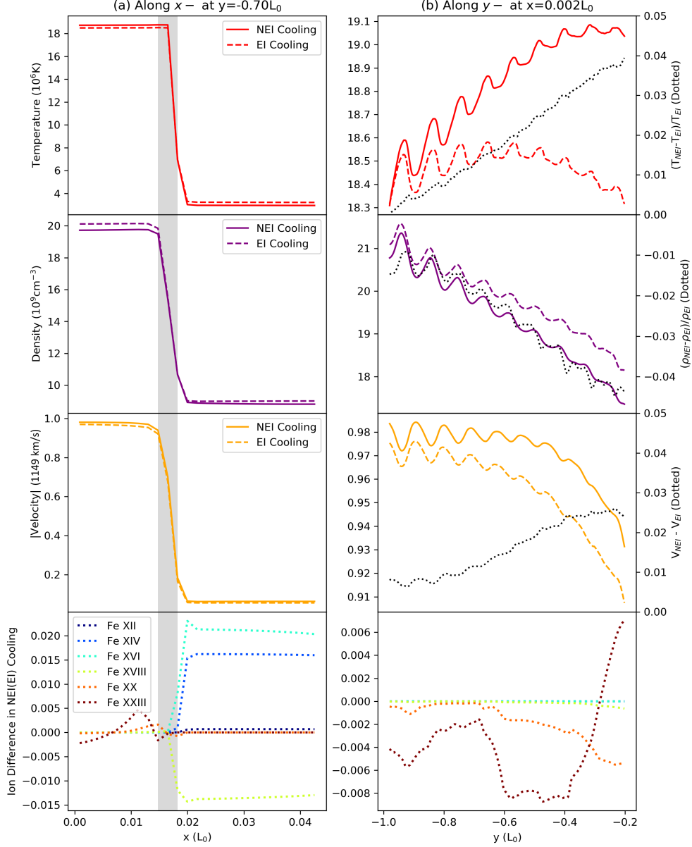
Figure 14. Comparison of primary variables and ion charge states between the NEI-dependent radiative cooling case (solid lines) and the EI-dependent cooling (dashed lines). (a) Temperature, density, and plasma flow velocity along reconnection inflow direction ( x- ) at y = -0.7L_0 . The vertical gray shadows indicate the position of the shock front, and the reconnection X-point is located at [x = 0, y = 0] as discussed in above Figure 1. The bottom panel shows Fe ion fraction differences defined by f_{i,\text{NEI cooling}} - f_{i,\text{EI cooling}} . (b) Similar to (a) but along the reconnection outflow direction ( y- ) at x = 0.002L_0 . The right axis of each panel shows differences between the two cases for temperature, density, and velocity profiles, respectively.
