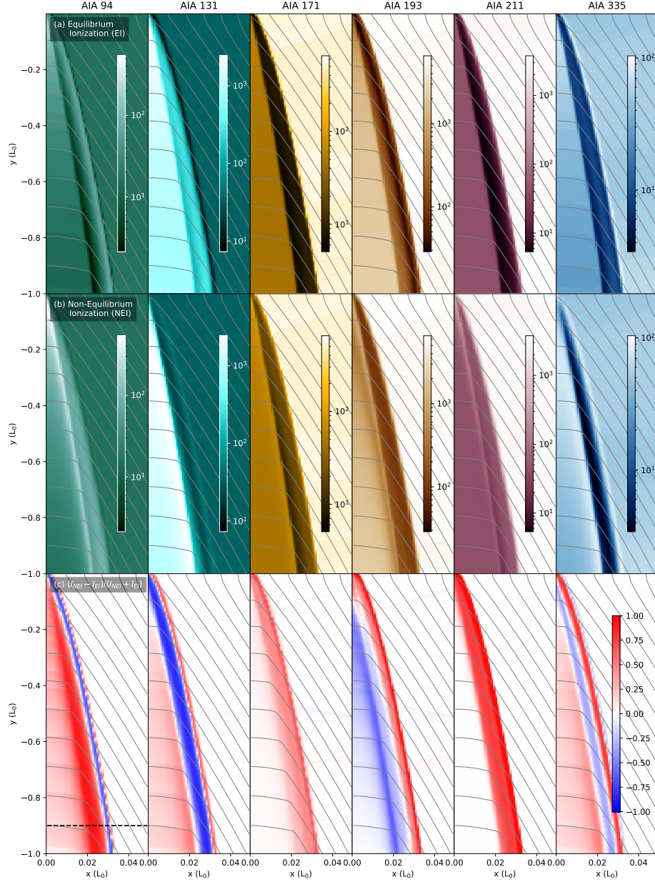
Figure 5. Synthetic SDO/AIA images for Case A2* with classical Spitzer thermal conduction coefficient. Row (a) and (b) are total count rates ( \text{DN s}^{-1} \text{ pixel}^{-1} ) for the equilibrium ionization and NEI results, respectively. (c) shows the relative difference (I_{nei} - I_{ei})/(I_{nei} + I_{ei}) between NEI and EI count rates.
